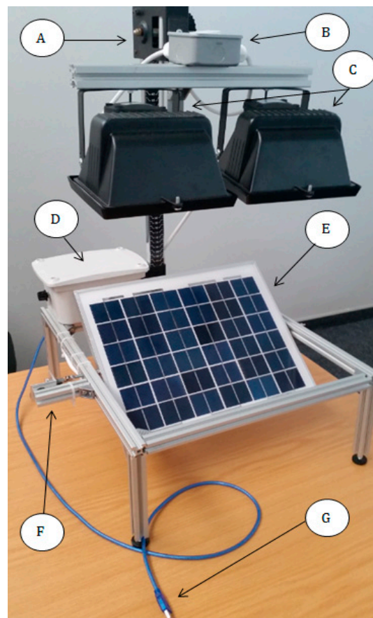
Figure 2. Innovative jig.
